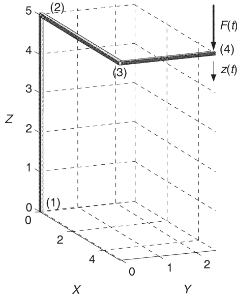
Fig. 8 Frame under pulse loading.
