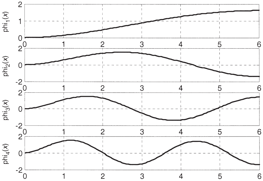
Fig. 5 Beam vibration modes.
