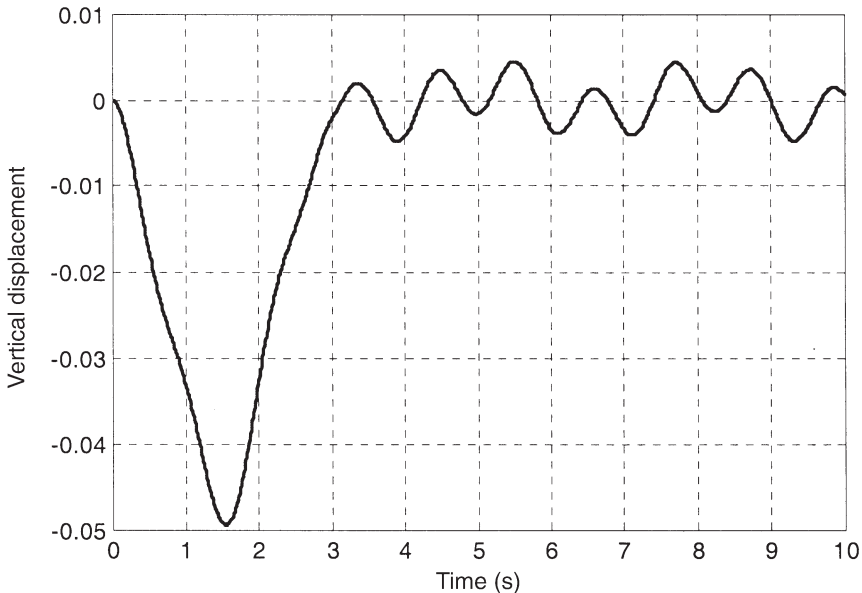
Fig. 9 Displacement of node 4.
